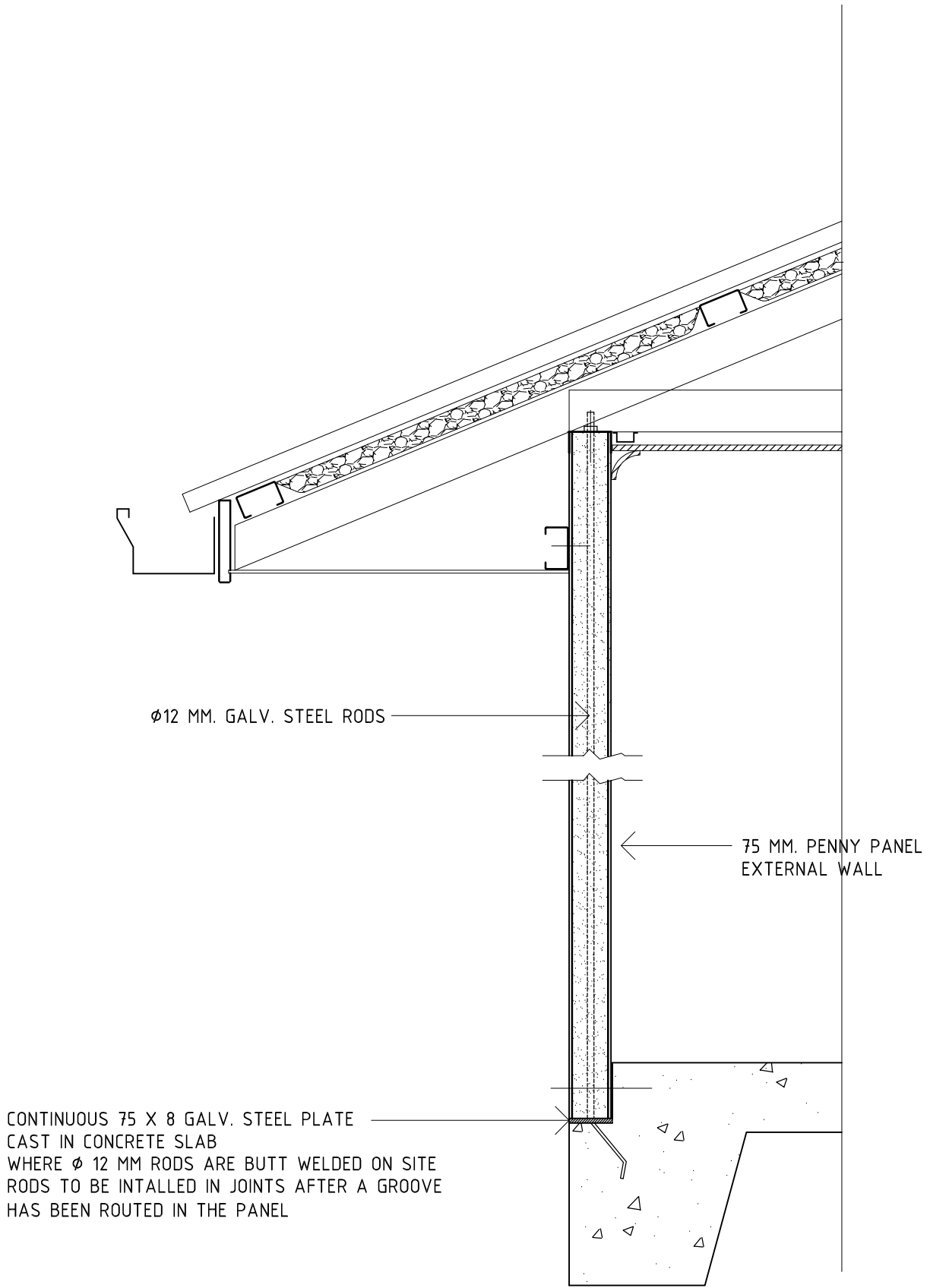
TYPICAL DOMESTIC CONSTRUCTION SECTION SHOWING WIND RODS INSTALLATION
