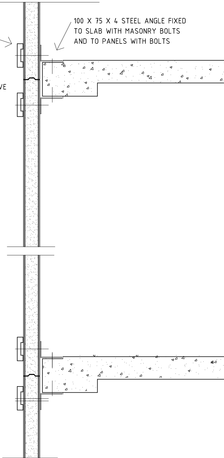
SECTION OF EXTERNAL PANEL ON REINFORCED CONCRETE STRUCTURE FOR CONTINUOUS PANEL FACADE
