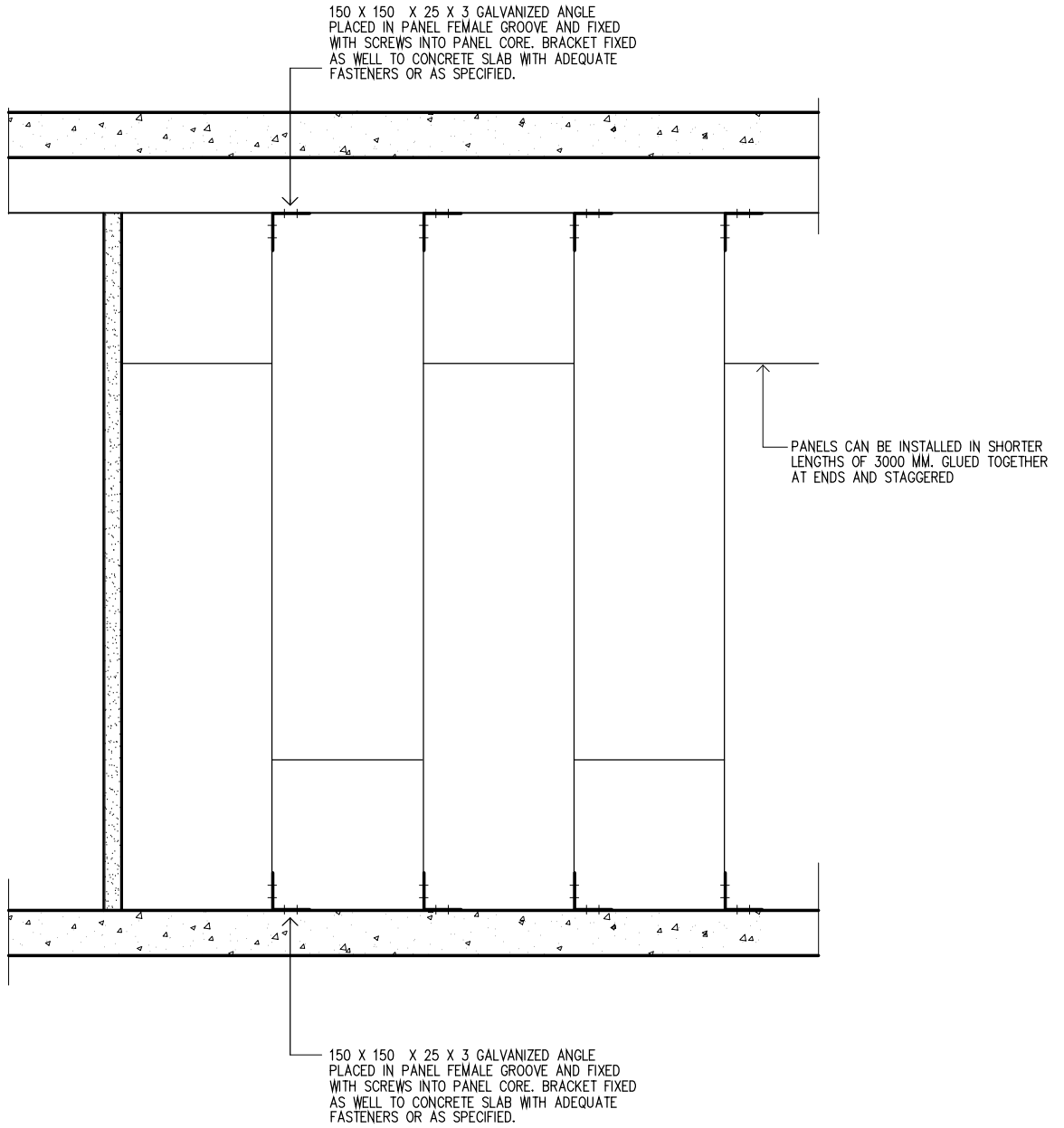
ELEVATION OF EXTERNAL PANEL ON AN EXISTING STRUCTURE FIXED WITH L SHAPED BRACKETS
