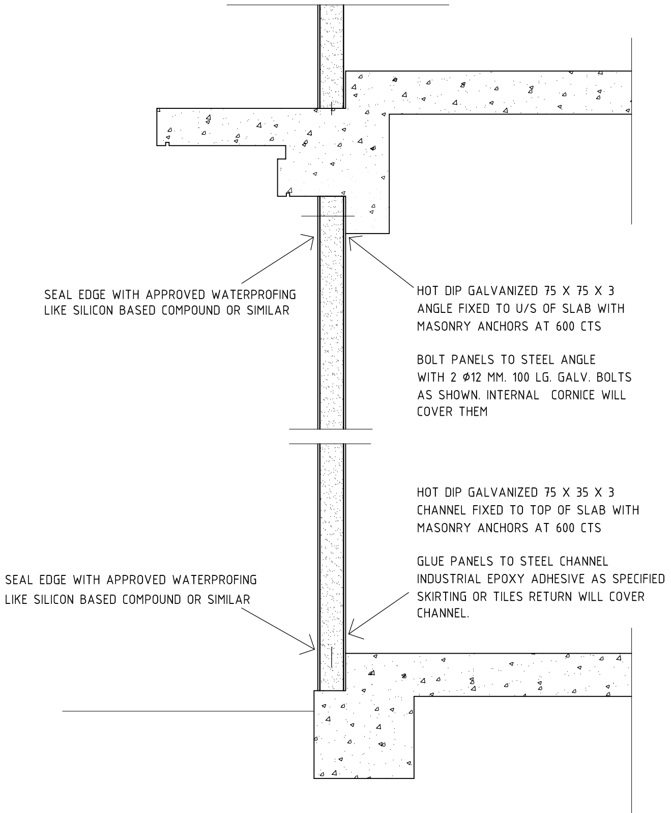
SECTION OF EXTERNAL PANEL ON AN EXISTING STRUCTURE FIXED WITH BOLTS TO CONCRETE SLAB
