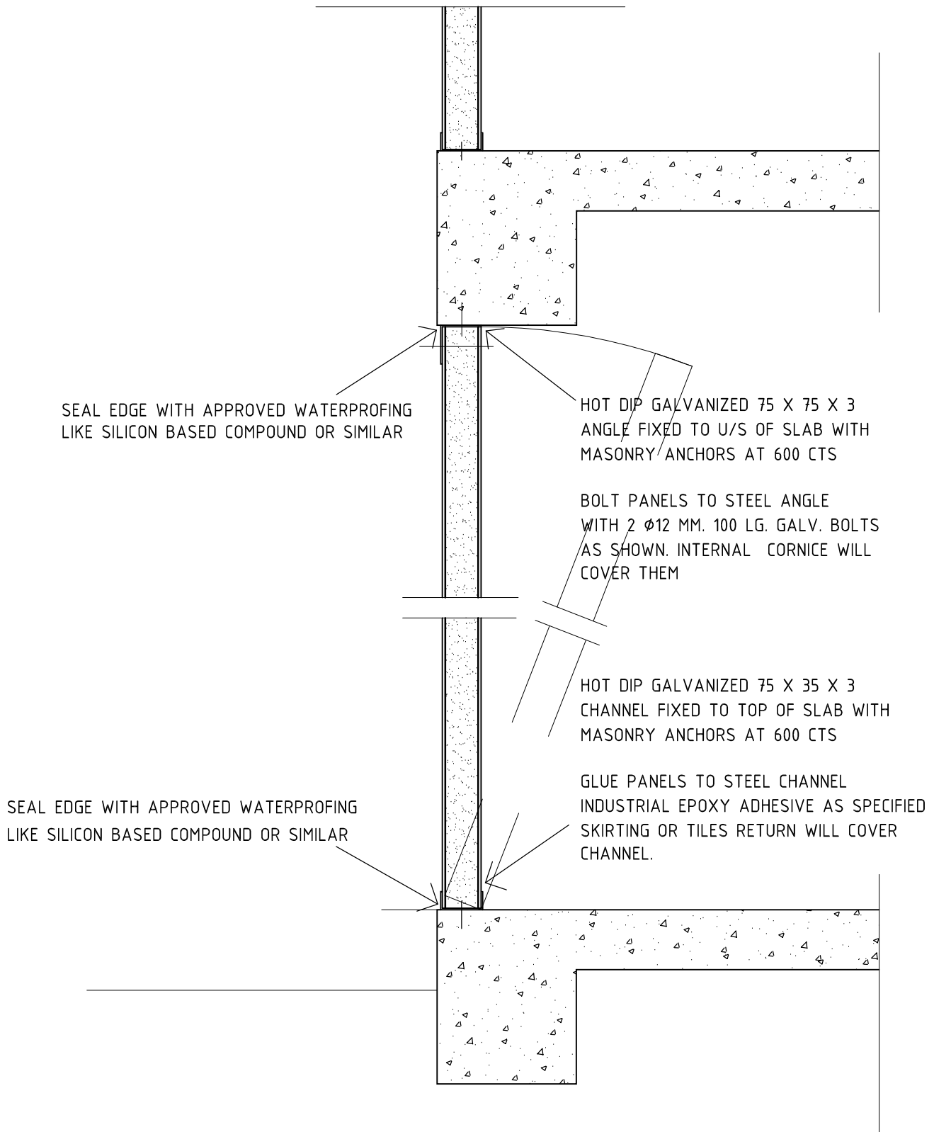
SECTION OF EXTERNAL PANEL ON AN EXISTING STRUCTURE FIXED WITH ANGLE AND STEEL CHANNEL
