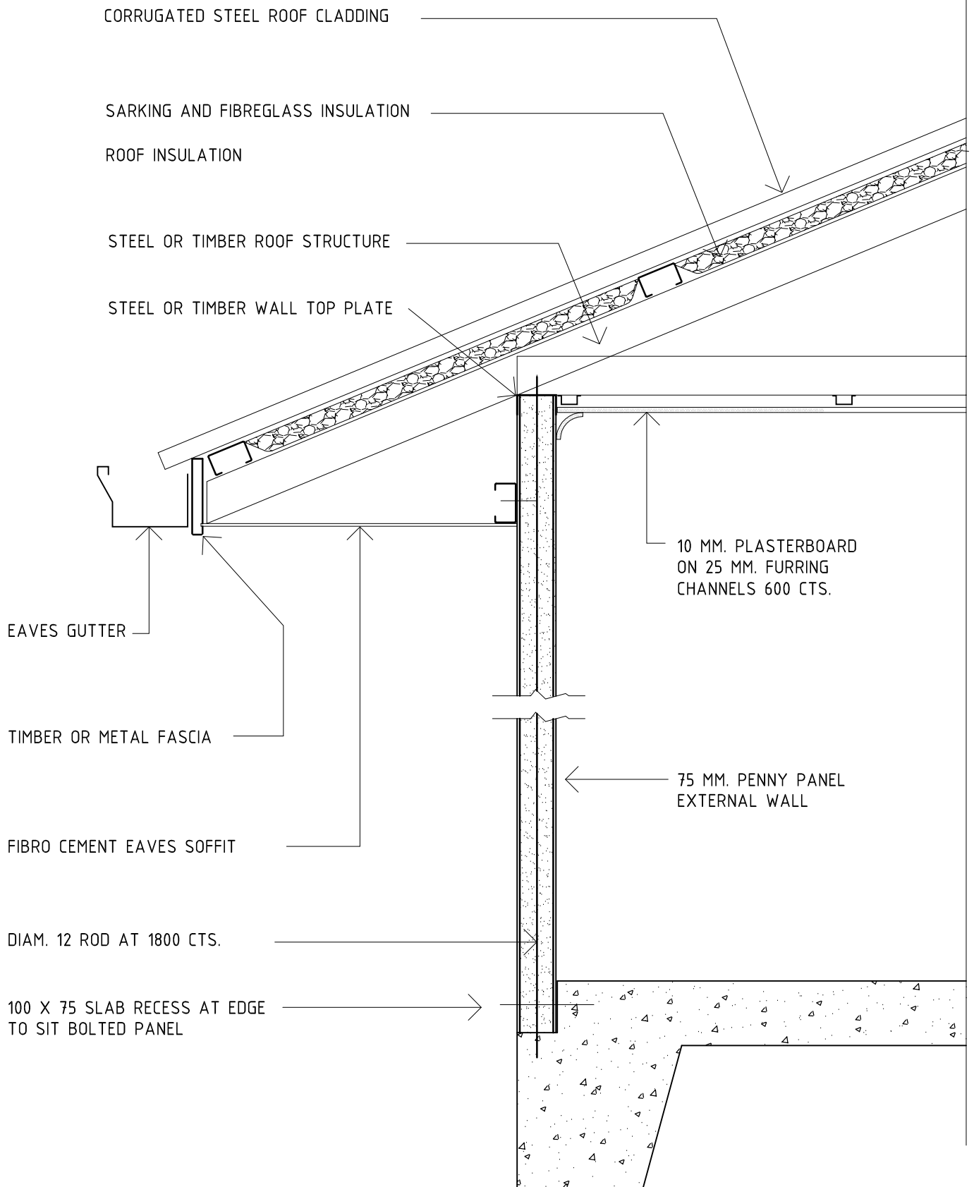
TYPICAL DOMESTIC CONSTRUCTION SECTION OF EXTERNAL WALL AND SLAB
