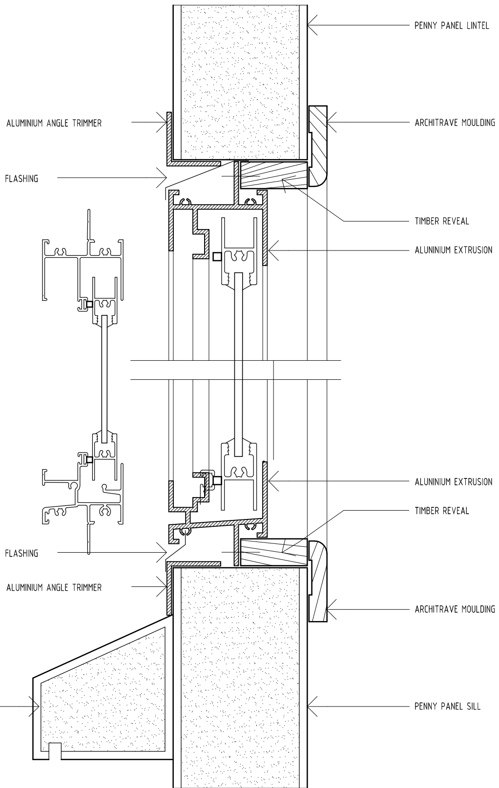
SCHEMATIC VERTICAL SECTION THRU ALUM. WINDOW WITH SILL
